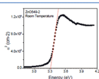
Fig. 4b Tauc plot to obtain the optical band gap for the 820 °C sample.
