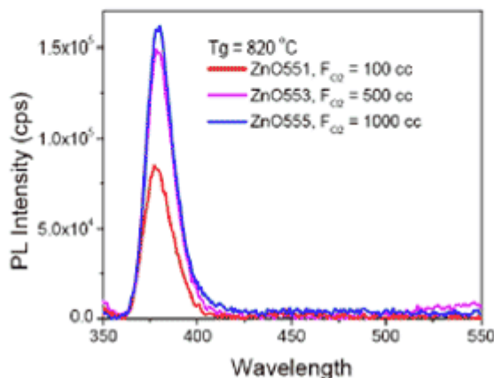
Fig. 6 PL spectra from the three samples with the different O 2 flow rate as indicated in the figure.
